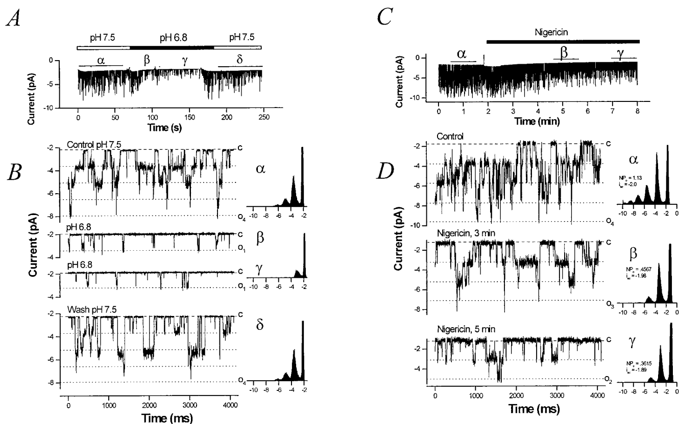
FIGURE 7. Intracellular acidosis inhibits the BLM K_{ATP} channel. (A and B) Lowering pH_i decreases channel activity in inside-out patches. In this inside-out experiment, the pipette contains KCl (solution d ), the bath contains NaCl (solution c ) plus 0.2 mM ATP, and the command potential is -60 mV. (A) The running average of current versus time (16-ms window) is shown. When the pH of the bath was lowered from 7.5 to 6.8, channel activity was inhibited by 79% ( nP_o changes from 0.67 to 0.14). This effect is reversible upon returning the bath pH to 7.5. (B) Original current traces representative of channel activity during the control period ( pH_i = 7.5 , top ), during acidosis ( pH_i = 6.8 , middle ), and after returning to pH_i = 7.5 ( bottom ). The all channels closed level ( dashed line ) and open channel levels ( dotted lines ) are indicated. (C and D) Lowering pH_i with nigericin decreases channel activity in cell-attached patches. In this cell-attached experiment, the pipette contains KCl (solution d ), the bath contains NaCl with 2.5 mM KCl (solution c ) plus 0.2 mM ATP, and the command potential is -80 mV. (C) The running average of current versus time (16-ms window) is shown. When nigericin ( 10 \mu M ) was added to the bath, channel activity was progressively inhibited. nP_o was reduced by 68% after 8 min in nigericin. (D) Original current traces and amplitude histograms representative of channel activity during the control period ( top trace ) and during nigericin ( bottom two traces ). The all channels closed level ( dashed line ) and open channel levels ( dotted lines ) are indicated.
