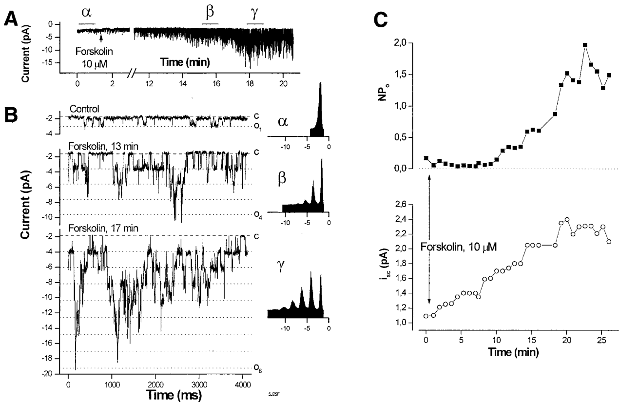
FIGURE 1. cAMP agonists activate the BLM K_{ATP} channel. (A) Forskolin (10 \mu M) activates the BLM K_{ATP} channel in cell-attached patches. In the experiment depicted, the pipette contains KCl (solution d ), the bath contains NaCl (solution c ), and the command potential is -60 mV. A running average of current versus time (window width 16 ms) is shown. (B) Sample traces taken from within the regions marked \alpha , \beta , and \gamma in A. The corresponding amplitude histograms were taken for each region. After the addition of forskolin, channel activity increases ninefold ( nP_o increases from 0.17 to 1.46). Note the increase in the single channel current ( i_{sc} ) due to the hyperpolarization of the cell membrane as K^+ channels open over the BLM. The all channels closed level (dashed line) and open channel levels (dotted lines) are indicated. (C) Forskolin increases both channel activity ( nP_o ) and single channel current ( i_{sc} ). nP_o (■) and i_{sc} (○) as measured in the experiment described in A are plotted versus time. i_{sc} increases as K^+ channels on the BLM open. From the change in i_{sc} ( \Delta i_{sc} = -0.9 pA), the hyperpolarization ( \Delta V_m ) is \sim -40 mV. Note that the increase in i_{sc} precedes the increase in nP_o , consistent with other BLM K_{ATP} channels opening before those in the patch.
