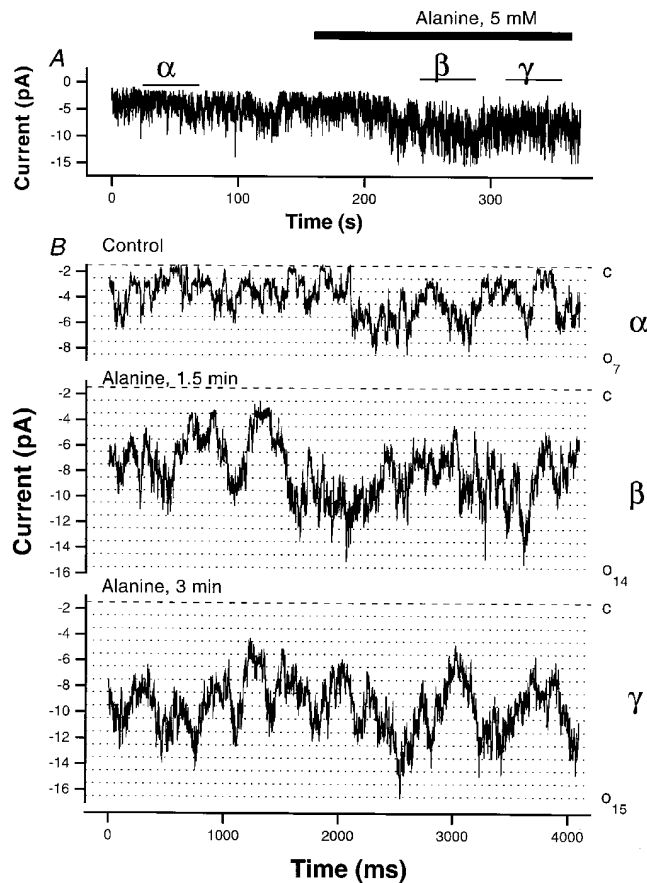
FIGURE 11. Stimulation of transport increases BLM K_{ATP} channel activity. (A) Activation of the Na^+K^+ -ATPase pump with substrates, in this case 5 mM alanine, results in an increase in activity of the BLM K_{ATP} channel in cell-attached patches. A running average of current versus time (16-ms window) is shown. The addition of alanine caused nP_o to increase nearly twofold (region marked \alpha : nP_o = 2.53 , region marked \beta : nP_o = 4.44 ). In this experiment, the pipette contains KCl (solution d ), the bath contains NaCl (solution c ), and the command potential is -60 mV. Sample traces taken from within the regions marked \alpha , \beta , and \gamma in A. Note that despite the opening of BLM K_{ATP} channels, the single channel current remains essentially constant due to a net balance of hyperpolarizing ( K^+ channel activation) and depolarizing ( Na^+ entry) forces. The all channels closed level (dashed line) and open channel levels (dotted lines) are indicated.
